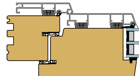
GS PREMIUM 200 HT
