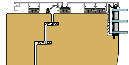
GS PREMIUM 510 HT
