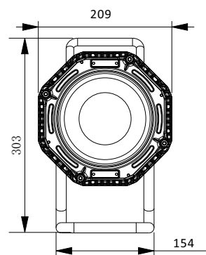
Item no.: 321174 FlutLED Ex 10W with floor frame
