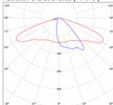
Radiation characteristics (147°/78°)
