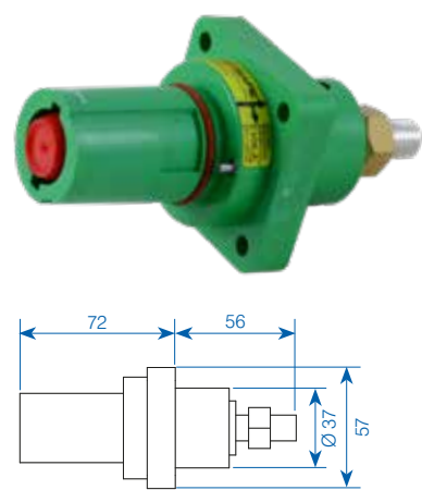
Plug-in connector
