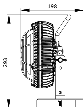
Item no.: 288400 FlutLED Ex 10W with magnetic base
