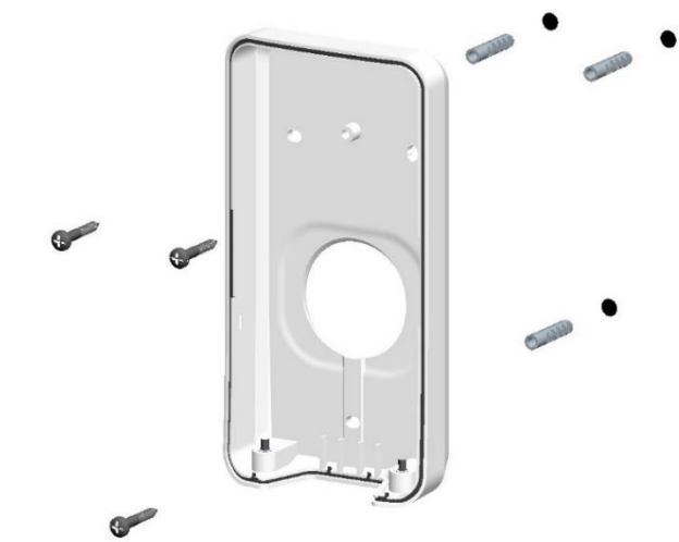
Figure 12: Fastening lower part
