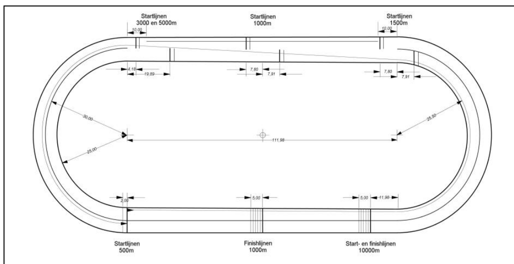
Standard layout for a 400 meter track
