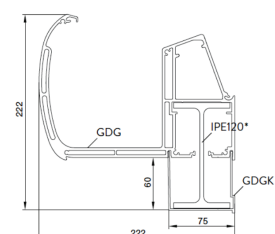
Gutter combination with reinforcement profile GDG + IPEI20* + GDGK
