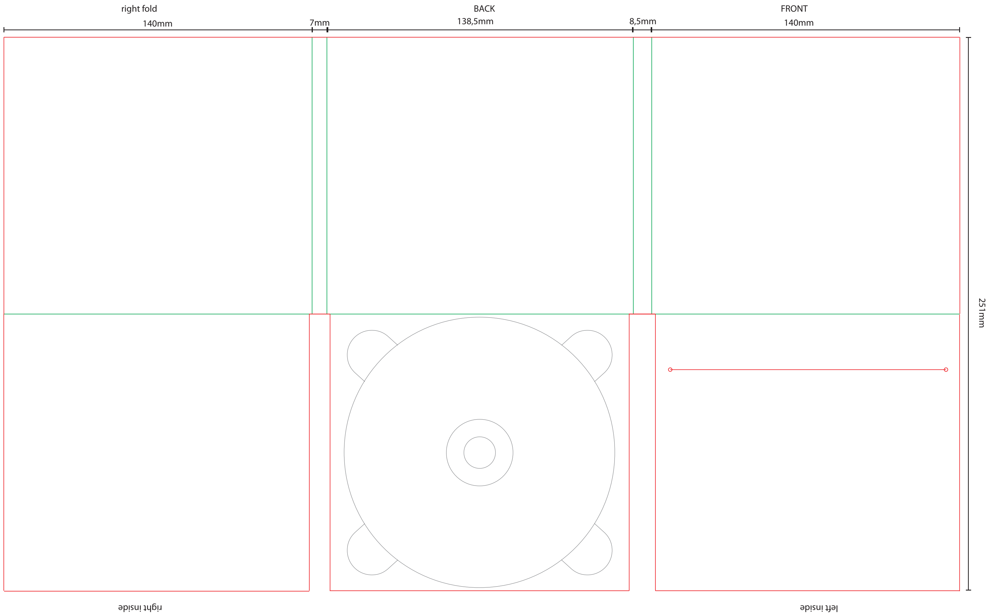
3-part CD digipack with digitray in the middle, booklet on the left side Template no: A-2346
