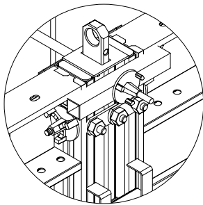
Fig. 7.7 - Cap - working position
