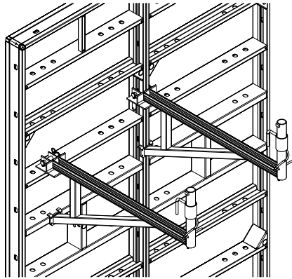
Fig. 3.25 – Sample method of installation of the working platform on the formwork
