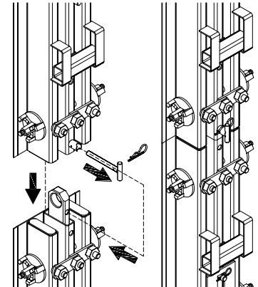
Fig. 7.9 - Joining formwork removing elements
