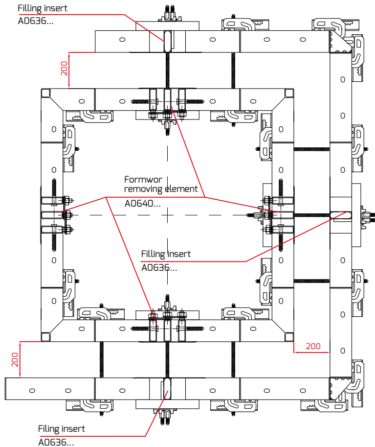
Fig. 7.3 – External set installation
