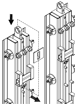
Fig. 7.8 - Cap repositioned
