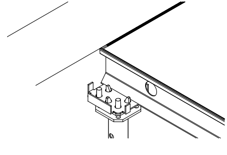
Fig. 14.9 – Prop - shoring head with the head cover located at the building wall
