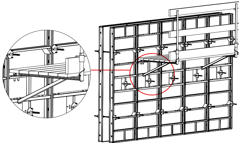
Fig. 3.24 – Sample installed working platform
