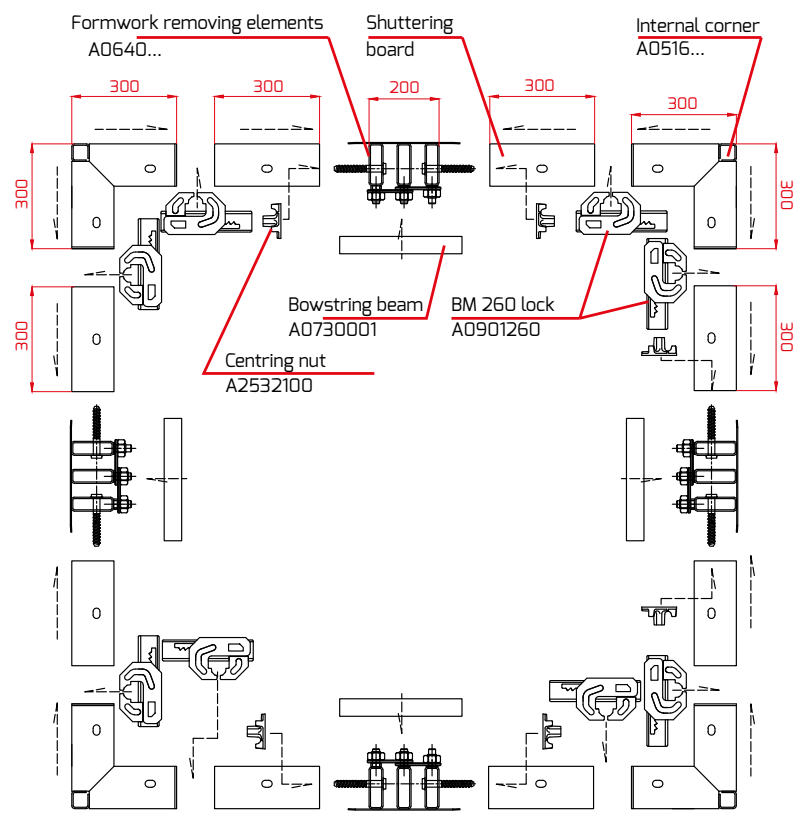
Fig. 7.2 – Diagram presenting the installation of the lift shaft formwork
