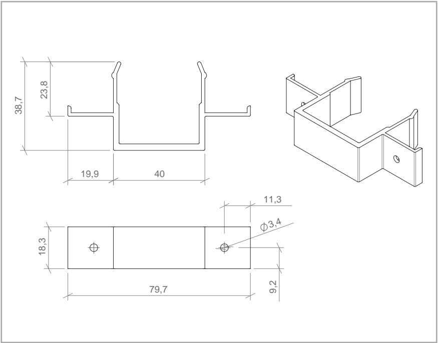
BRACKET STB-CH
