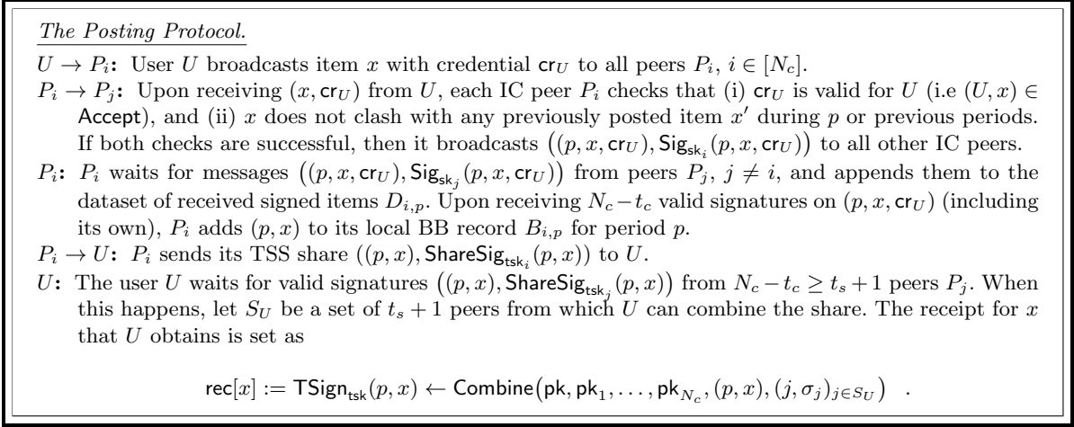
Fig. 6. The Posting protocol of the CS BB system during period p w.r.t. the posting policy \mathcal{P} = (\text{Accept}, \text{Select}(\cdot)) , for fault tolerance threshold of t_c out-of N_c IC peers P_1, \dots, P_{N_c} , and a (t_s, N_c) -TSS. Selection function \text{Select}(\cdot) is the identity function.
