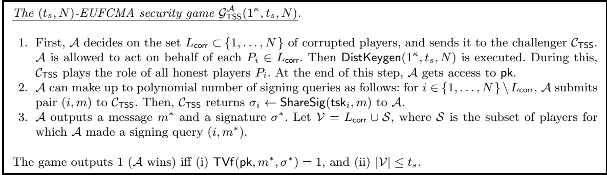
Fig. 2. The (t_s, N) -EUFMA security game \mathcal{G}_{\text{TSS}}^A(1^\kappa, t_s, N) between the challenger \mathcal{C}_{\text{TSS}} and the adversary \mathcal{A} .
