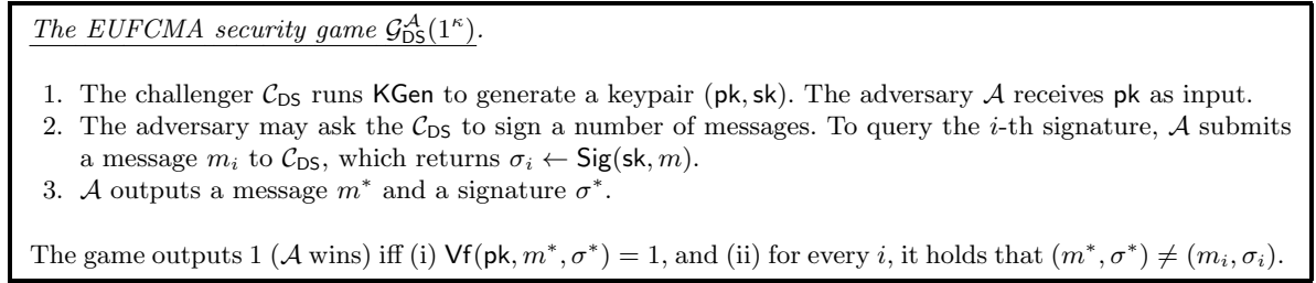
Fig. 1. The EUFCA security game \mathcal{G}_{\text{DS}}^A(1^\kappa) between the challenger \mathcal{C}_{\text{DS}} and the adversary \mathcal{A} .
