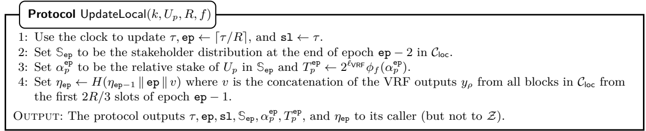
Fig. 8. The protocol for updating the local stake distribution parameters.
