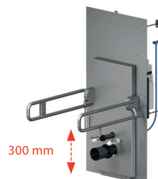
AM101/1500L Medic Assistant Pre-wall installation system for dry build up, height adjustable – for people with reduced mobility
