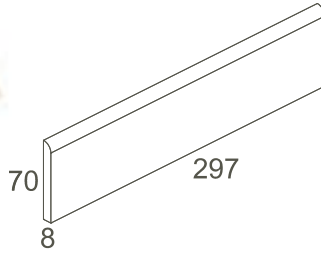
Süpürgelik Plinth M 7 x 30 cm / 3" x 12" 70 x 297 x 8 mm EN14411 Bla
