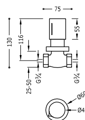
Concealed shut-off valve Female thread connection: 3/4". Chiave d'arresto a incasso Attacco a filetto femmina: 3/4".
