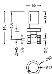
Concealed shut-off valve Female thread connection: 1/2". Chiave d'arresto a incasso Attacco a filetto femmina: 1/2".
