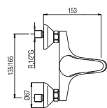
Monocomando vasca Doccetta anticalcare con supporto orientabile. Flessibile doppia graffatura Single lever bath and shower mixer Anti-limescale hand shower with directable support. Double interlocked shower hose
