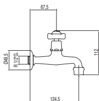
Rubinetto office Kitchenette tap Kuchyňská baterie
