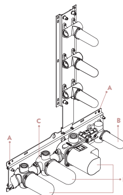
block system® horizontal
