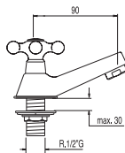
Rubinetto lavabo da 1/2" 1/2" basin pillar tap Umyvadlová baterie 1/2"
