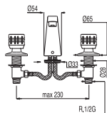
Accumulatore lavabo Wash-basin mixer Umyvadlová baterie
