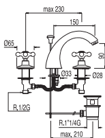
Accumulatore lavabo Wash-basin mixer Umyvadlová baterie
