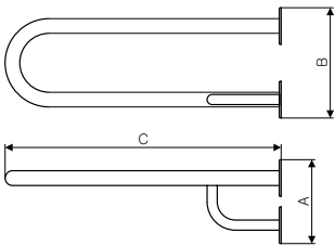
• Drawing for the left hand side version.
