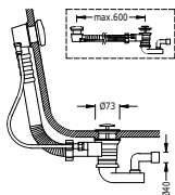
Bath drain with overflow and pop-up waste Ø 73 mm
