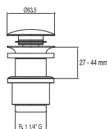
Valve for basin Ø 63,5 mm CLICK-CLACK (27-44 mm.)
