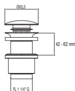
Valve for basin Ø 63,5 mm CLICK-CLACK (42-62 mm.)
