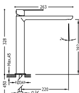
Single lever washbasin mixer with base extension
