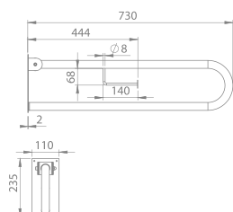
Hinged Grab Bar With Roll Holder 9AD0731031
