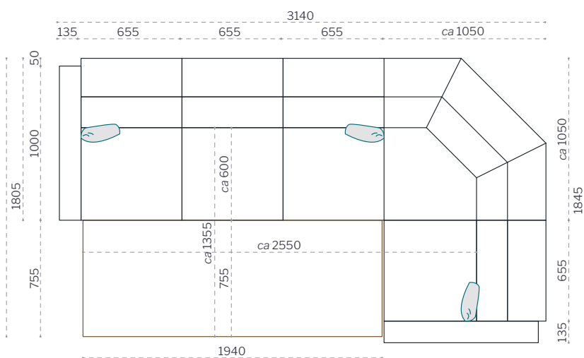
top view / 3-seater + corner + 2-seater
