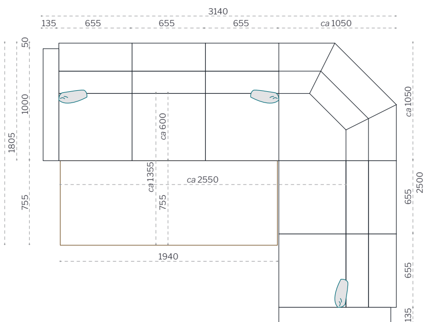
top view / 3-seater + corner + 2-seater
