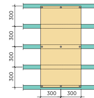
Impact resistance class 1A, 1200 x 600 mm panel fastened with 9 screws
