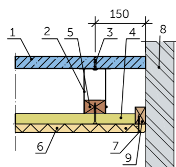
Node 2. Joint between longitudinal edges
