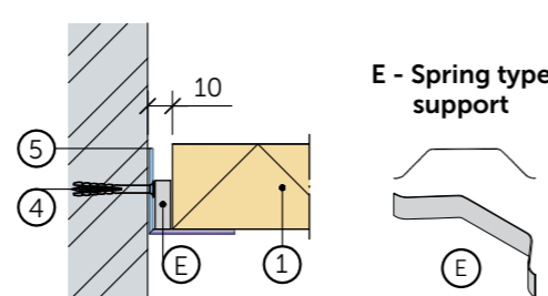
Supporting perimeter with wall L profile L35x35 mm
