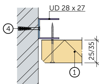
Fastening on perimeter metal profile
