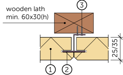
CEWOOD clip fastening on wooden lath
