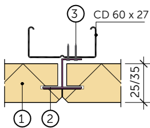
CEWOOD clip fastening on CD profile
