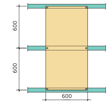
Impact resistance class 2A, 1200 x 600 mm panel fastened with 6 screws
