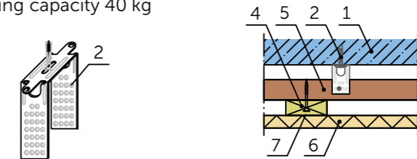
Joint between longitudinal edges
