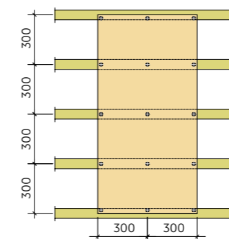
1200 x 600 mm panels fasten with 15 screws
