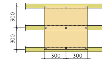
600 x 600 mm panels fasten with 9 screws
