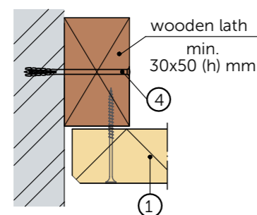
Fastening on perimeter wooden lath
