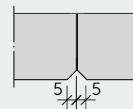
CEWOOD short edge profile P5
