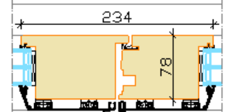
Mullion
