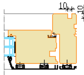
Jamb with extension
