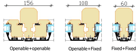
Openable+openable
