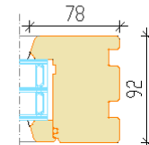
Fixed window
