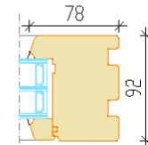
Fixed window
