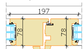
Middle part of double door
