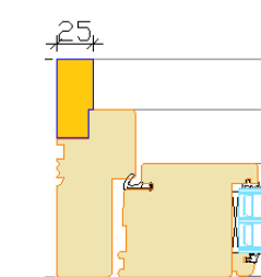
Jamb with extension
