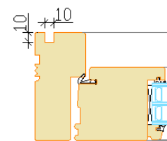
Jamb with Groove
