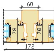
Openable+Openable
