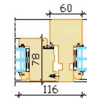
Openable+Fixed
