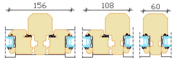
Openable+openable
