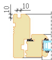
Grooved frame
