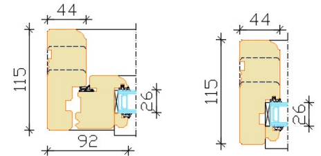
Openable window
