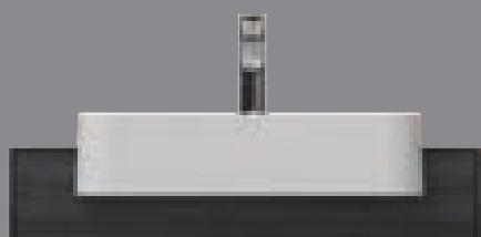
Marino Basin Unit 80 cm 800 x 220 x 490 mm
