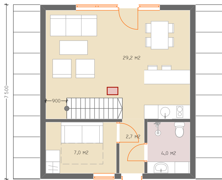
1FLOOR
