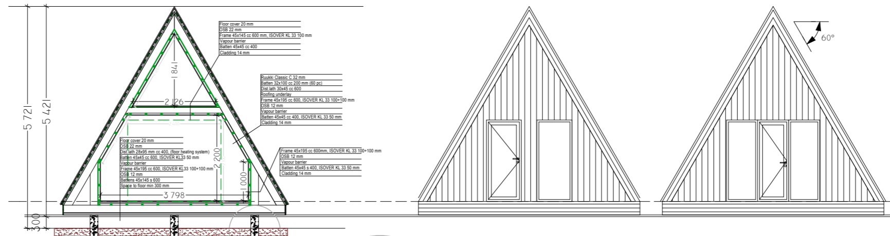
SECTION
