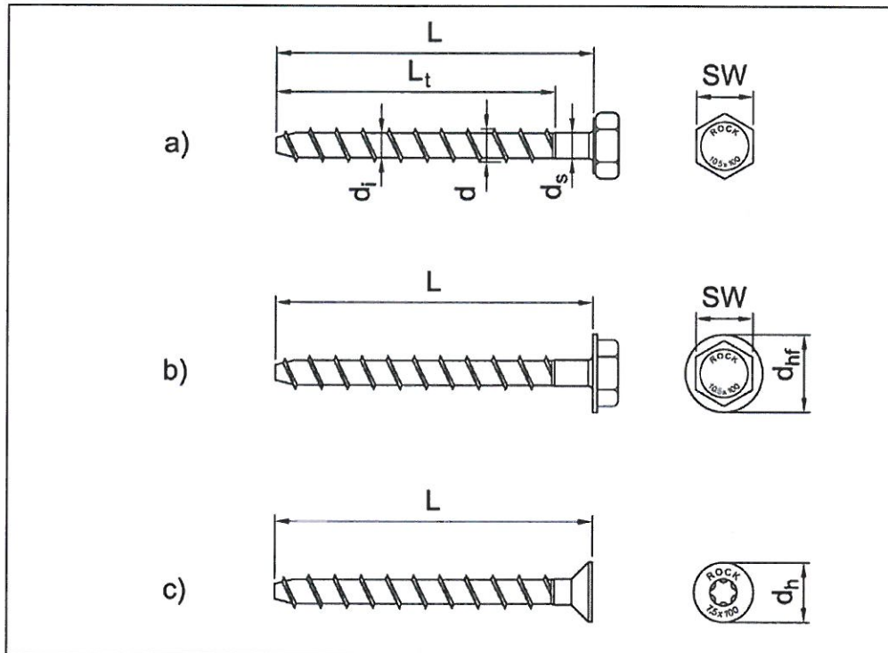
Screw types: a) BeziFix Anker hexagon head 7,5, 10,5 and 12,5. b) BeziFix Anker hexagon head with flange 7,5, 10,5 and 12,5. c) BeziFix Anker countersunk head 7,5. Head marking: "Rock" and size x screw length.
