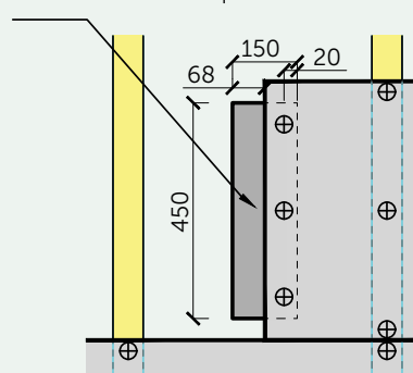
Option 3 - with connecting timber plate. (wind pressure <1kN/m 2 )
