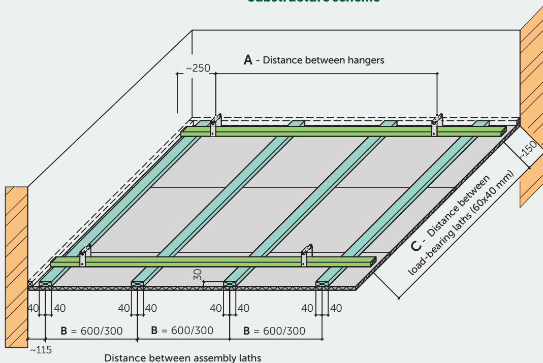
Substructure scheme
