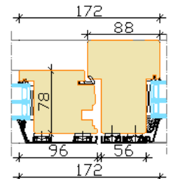
Mullion
