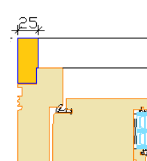
Jamb with extension
