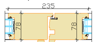
Middle part of double door
