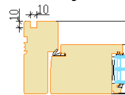
Jamb with groove
